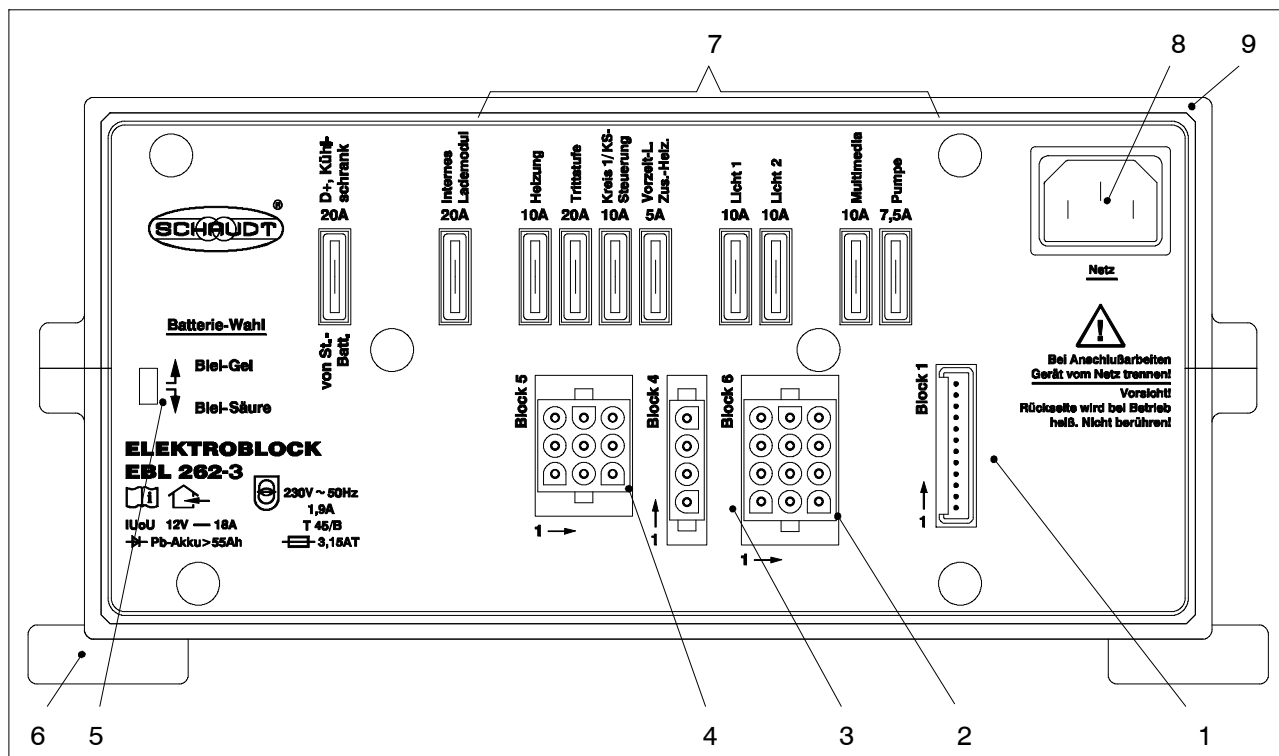
Fig. 3 Layout of the EBL 262-3 electroblock (front)
