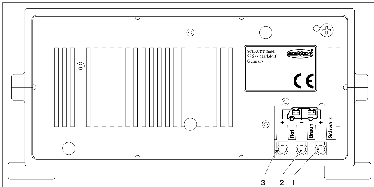
Fig. 4 Layout of EBL 262-3 electroblock (rear)
